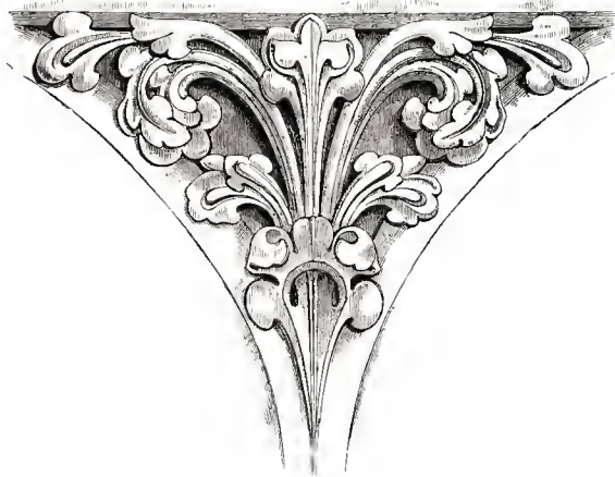
Wells Cathedral.—CORBELS.
